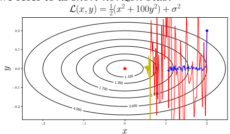
Figure 1: Aggressive learning rate (red) followed by a decay schedule (yellow) wins over conservative learning rate (blue) by making more progress along the low curvature direction ( x direction).
